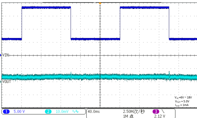
Line Transient
