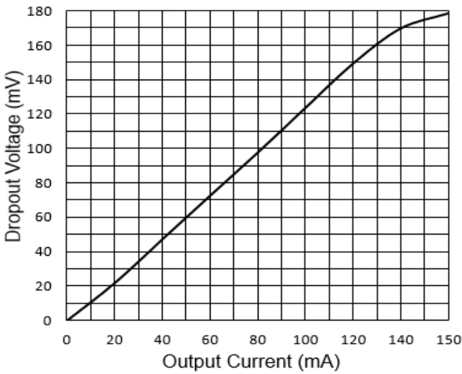
Dropout Voltage vs. Output Current ( V_{OUT} = 2.8V )
