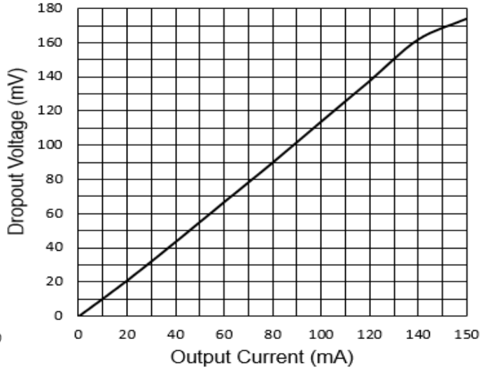
Dropout Voltage vs. Output Current ( V_{OUT} = 3.0V )
