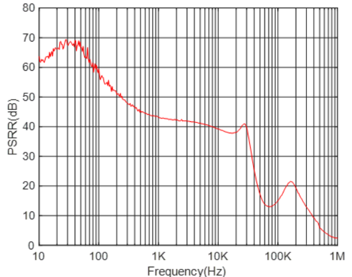
Power Supply Rejection Ratio vs. Frequency ( V_{OUT} = 3.0V )
