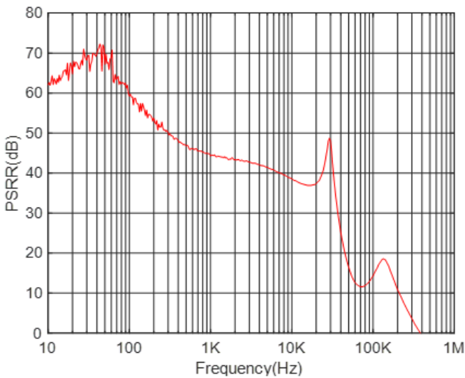
Power Supply Rejection Ratio vs. Frequency ( V_{OUT} = 2.8V )
