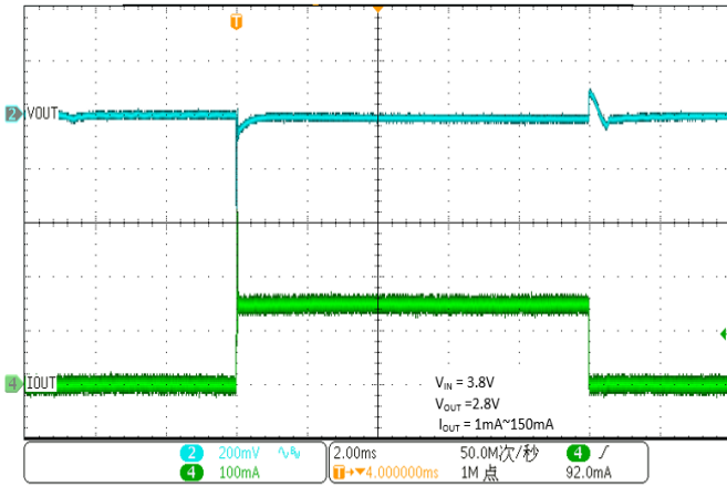
Load Transient
