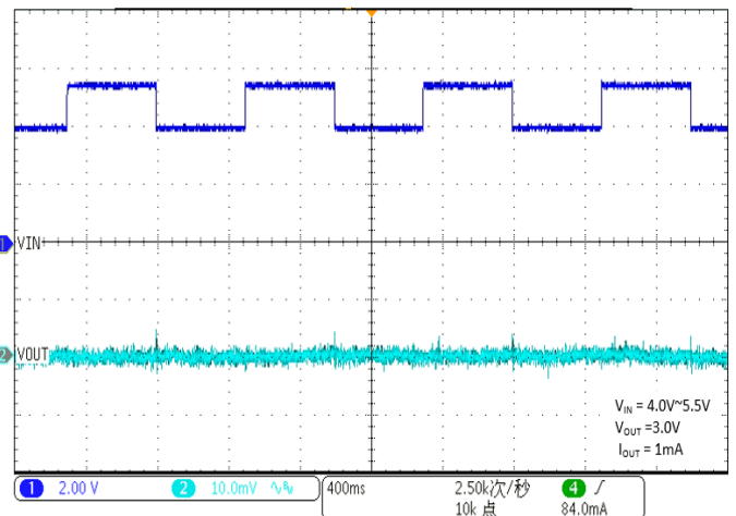
Line Transient
