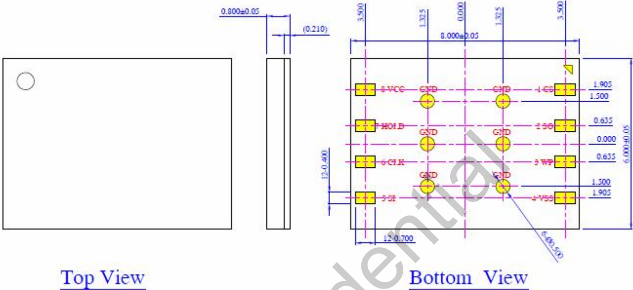
Figure 17-1 8 Pad WSON 6X8mm
