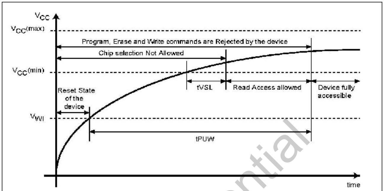
Figure 14-3 Power up Timing Sequence
