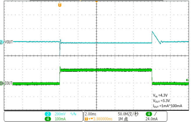
Load Transient
