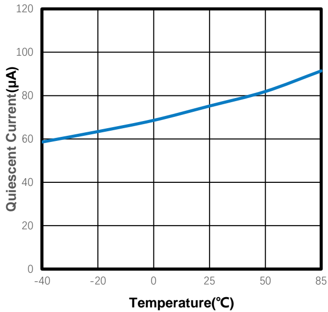
Figure 1. Quiescent Current vs. Ambient Temperature
