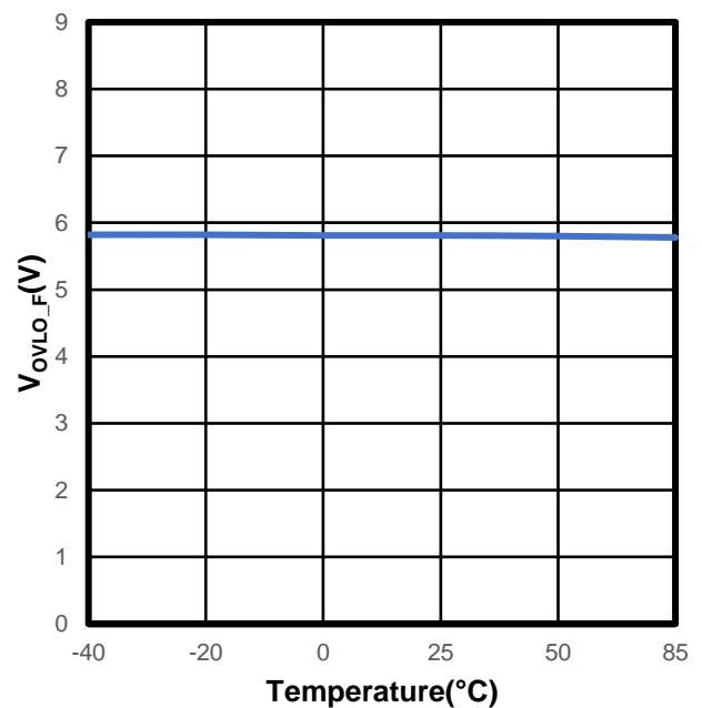
Figure 4. V_OVLO_F vs. Ambient Temperature
