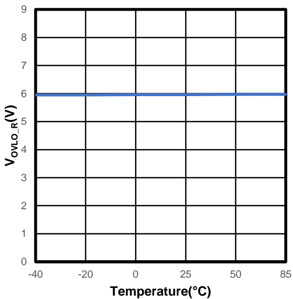
Figure 3. V_OVLO_R vs. Ambient Temperature
