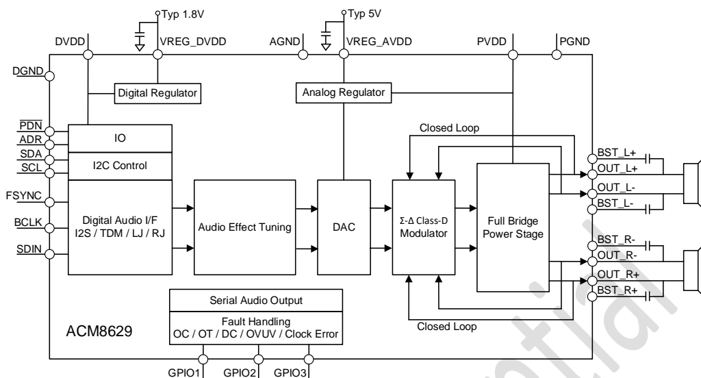
Figure 19 Function Block Diagram
