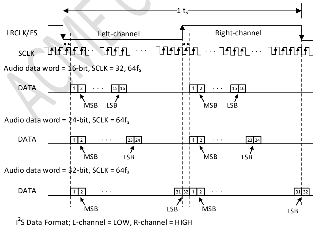
Figure 20 I 2 S Audio Data Format
