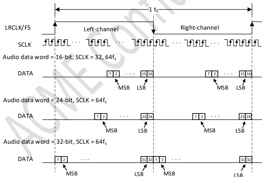
Figure 22 Right-Justified Audio Data Format
