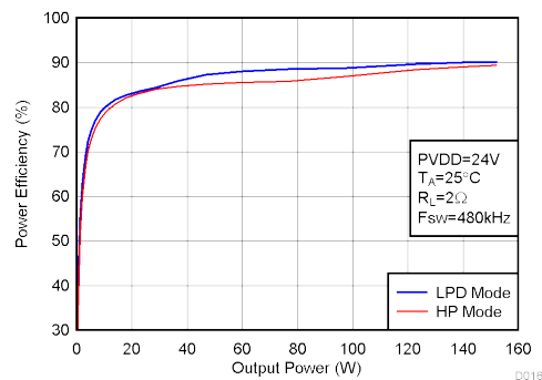
(Load=2Ω, Fsw=480kHz, LPD Mode)
