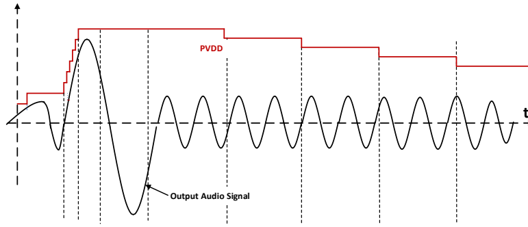
Figure 26 Class H Operation Signal
