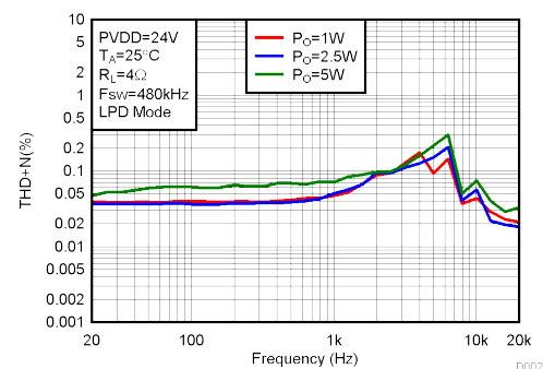
(PVDD=24V, Load=4Ω, Fsw=480kHz)
