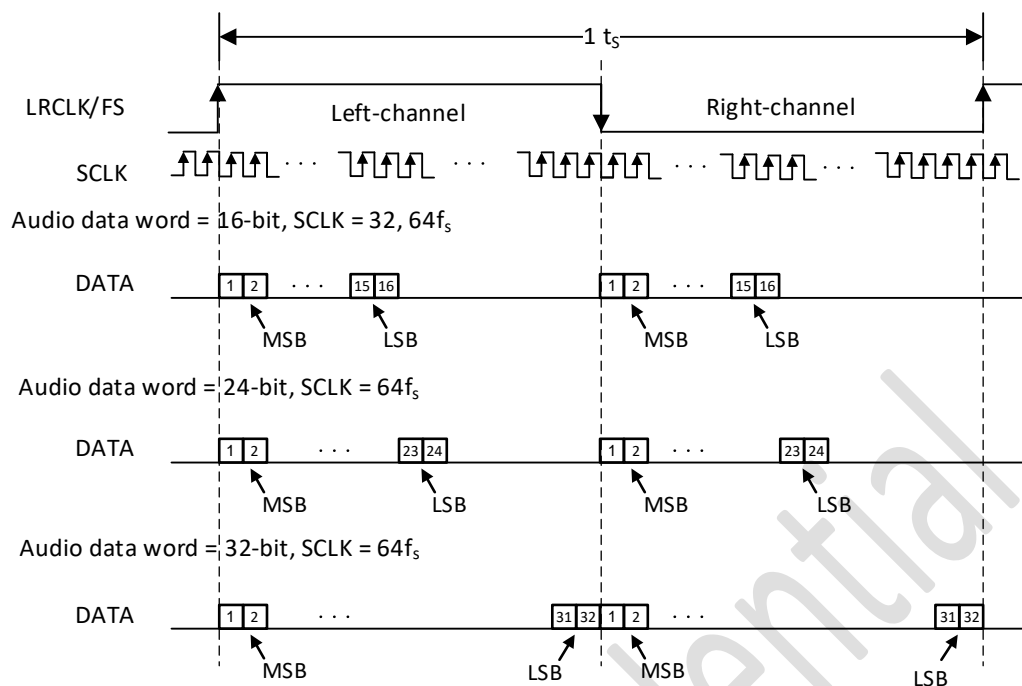
Figure 21 Left-Justified Audio Data Format
