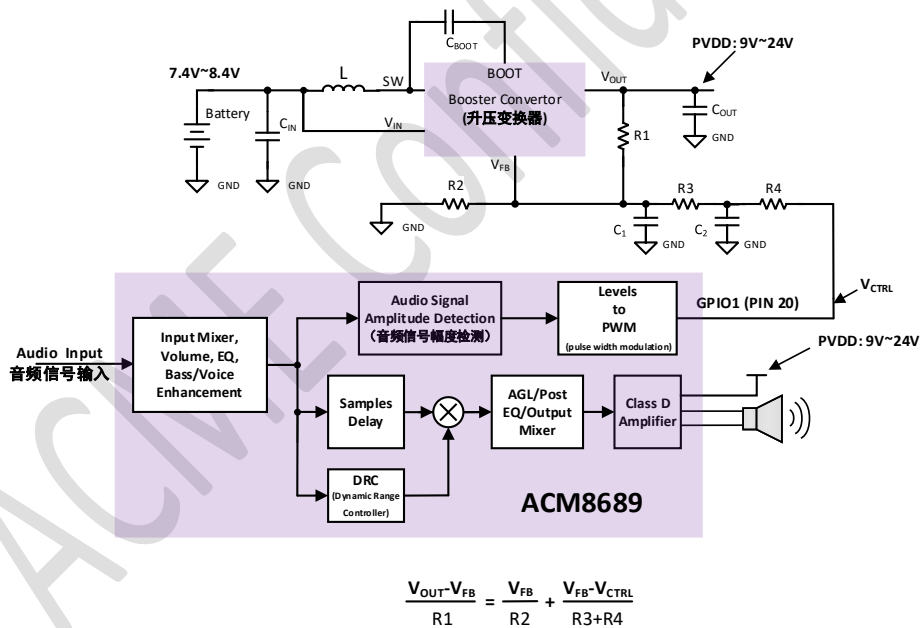
Figure 27 Class H Control Block
