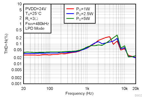
(PVDD=24V, Load=3Ω, Fsw=480kHz)
