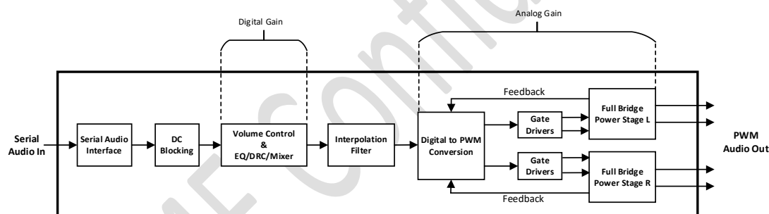
Figure 25 Gain Structure
