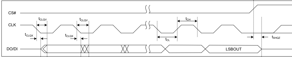
Figure 8.4 Serial Output Timing
